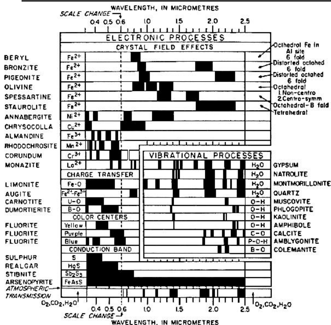
Figure 2 - Spectral signature diagram
