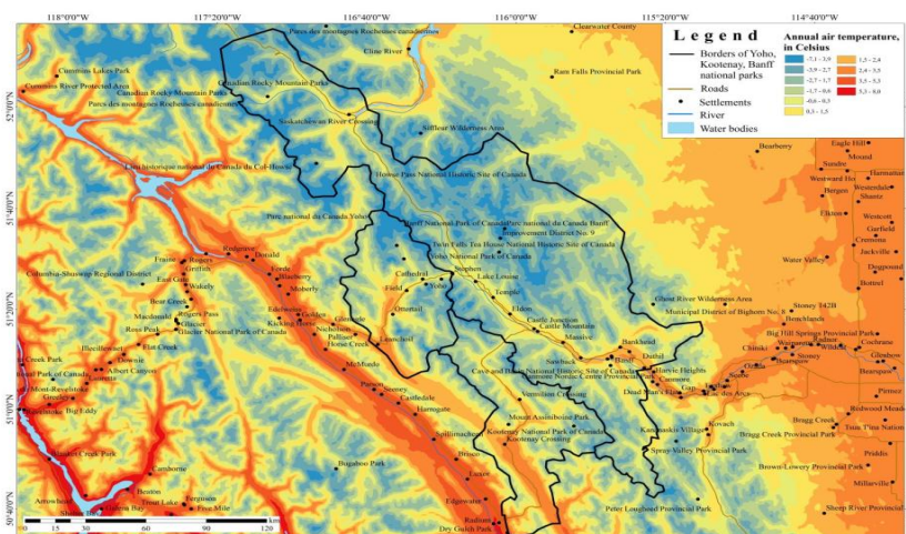
Fig. 5. Map of the average annual air temperature in Yoho, Kootenai, and Banff Parks (Canada). Compiled by the author
