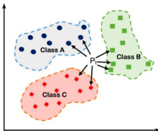
Figure 4 - The k-Nearest Neighbors
