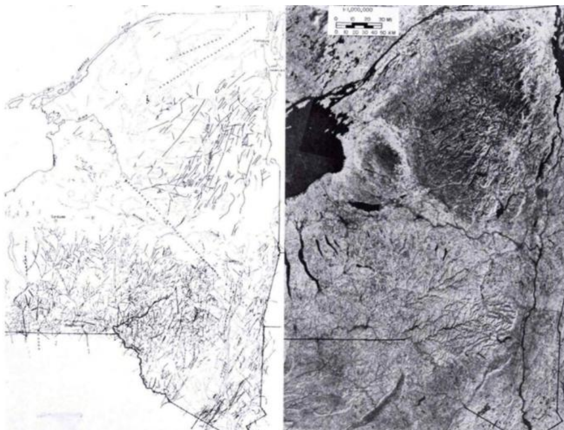
Figure 1 - LANDSAT mosaic and lineament map of eastern New York State (after Isachsen, 1973).
